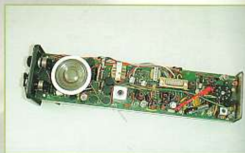
De print van de 30-40 MHz transceiver.
